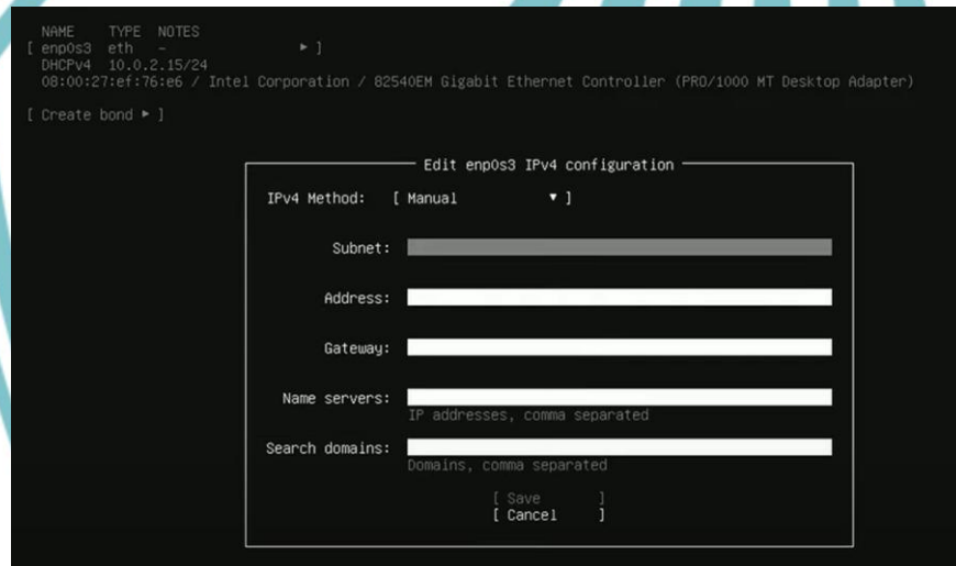
Gambar 4.12 Network Configuration Ubuntu
