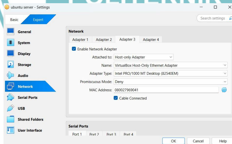
Gambar 4.6 Ubuntu Adapter Configuration
