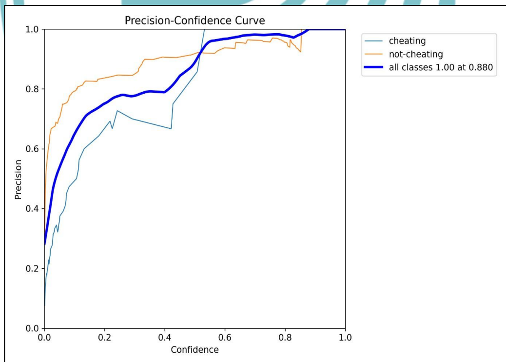
Gambar 11: Precision-Confidence Curve
