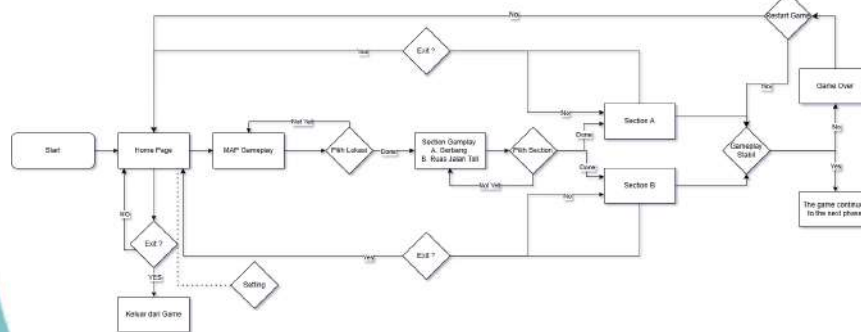
Gambar 4.1 Flowchart Game Toll Tycoon
