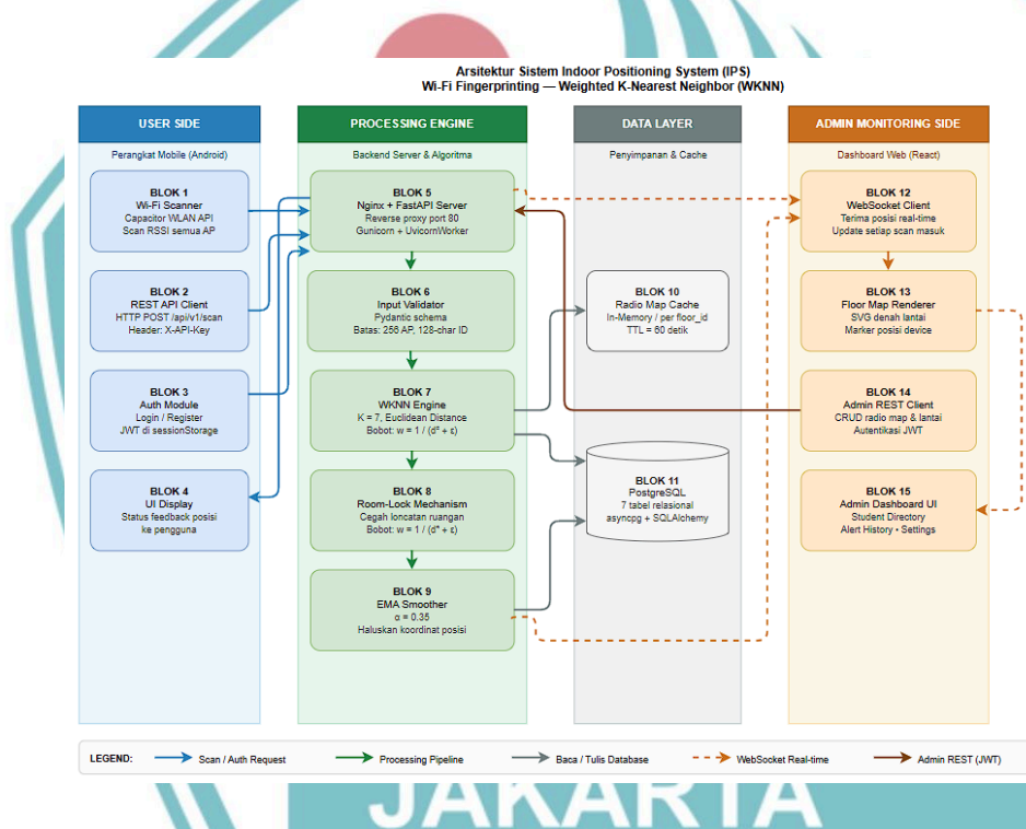
Gambar 3.2 Diagram Blok Arsitektur Sistem Indoor Positioning System
